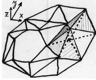
Fig. 5.4. Visual representation of one basis function on the mesh of the disk
