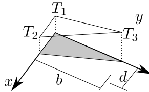
Fig. 6.7. Illustration of how a poorly shaped triangle can magnify errors in temperature to become large errors in temperature gradient
