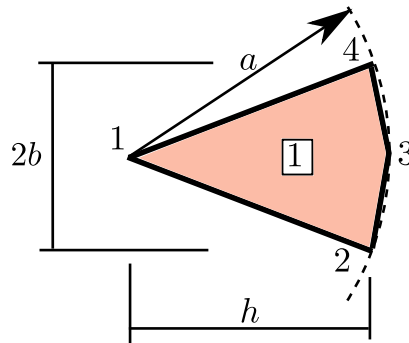
Fig. 4.3. Concrete column with prescribed zero temperature on the boundary and hydration heat source. Mesh with a single Q4 element.
